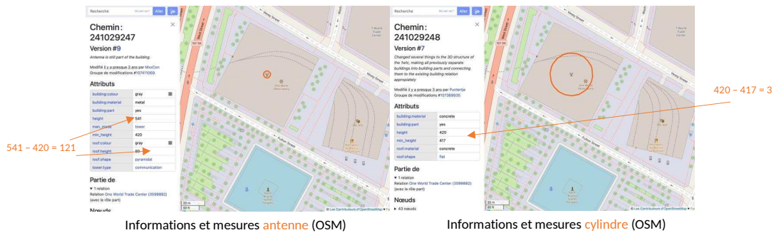
FIGURE 2.34 – Blender — OSM
