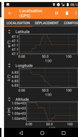
(e) Phypbox
